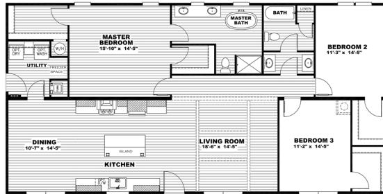
MODEL #PCH32603A DRAWING # 30M006 32'X60' THE BUFORD
